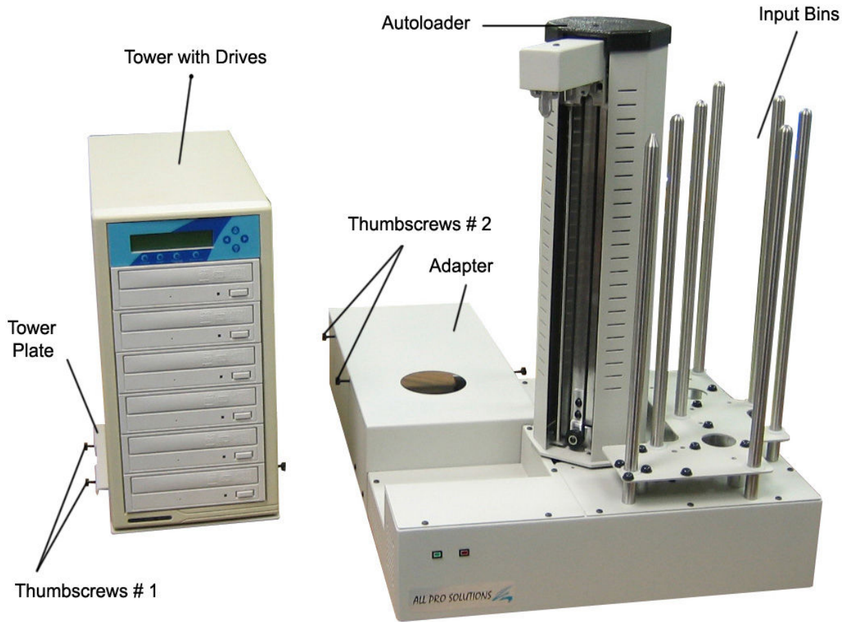
Fig.2 Tower alignment
