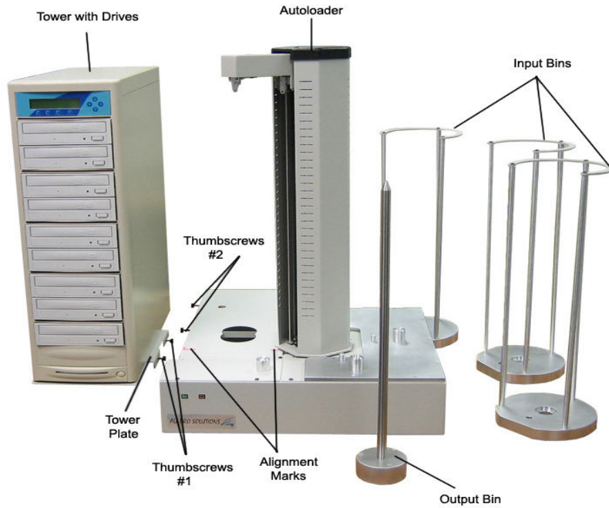
Fig. 5b HERA-9 (system assembled)
