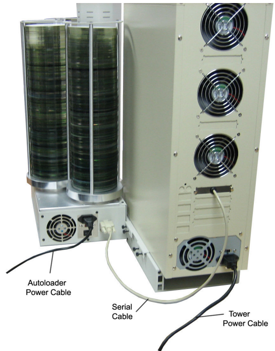
Fig. 5c HERA-9 (back view – cables)
